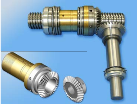
Rotary nut with paired bevel gears ratio 1:1 art.CFB/HR..+CC1:1
