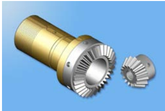
Rotary nut with paired Bevel gears ratio 1:2 art.CFB/HR..+CC1:2-SGR
